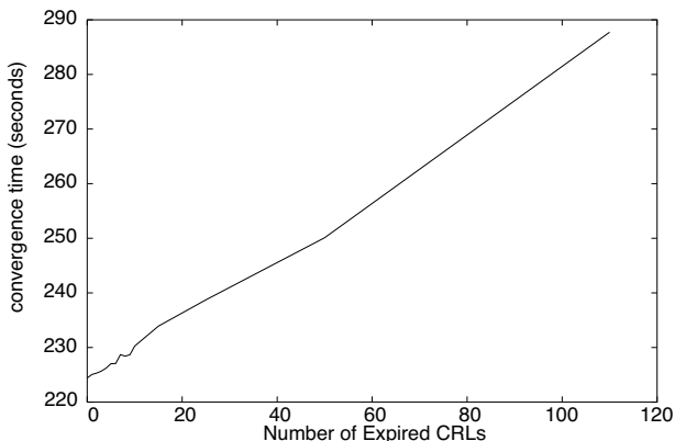
Figure 9: Convergence times by S-BGP using CRLs to validate certificates.
