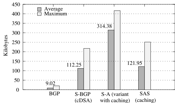
Figure 8: Comparison of memory costs for caching. The S-A scheme in this comparison is a variant that does not use hash trees, and caches leaf information instead of signatures.
