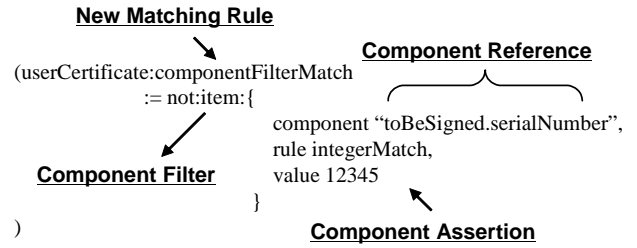
Figure 7. Example Component Filter.
